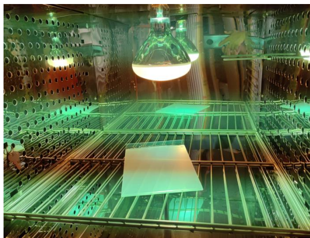
Flat type, just put the sample flat on the sample rack, irradiation degree depends on the distance
