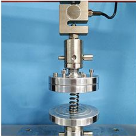
compress clamps
