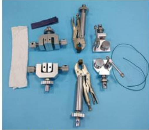
textile clamps
